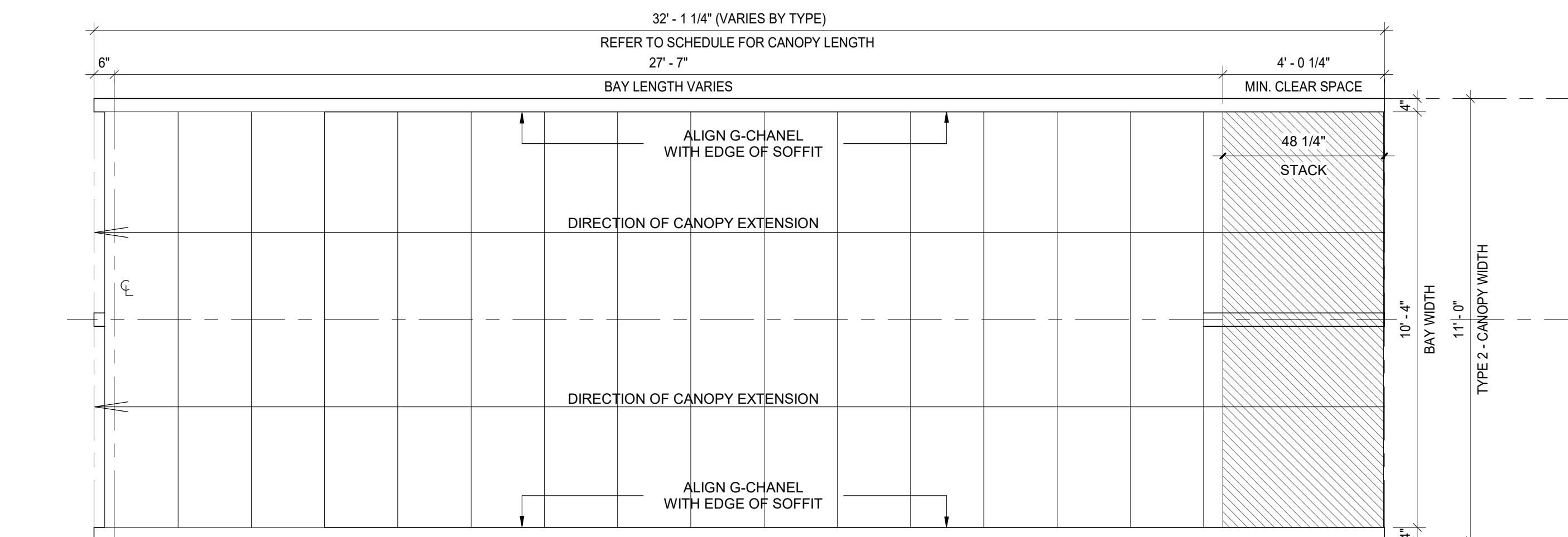
DETAIL - PLAN DIAGRAM - CANOPY TYPES 2 & 5
