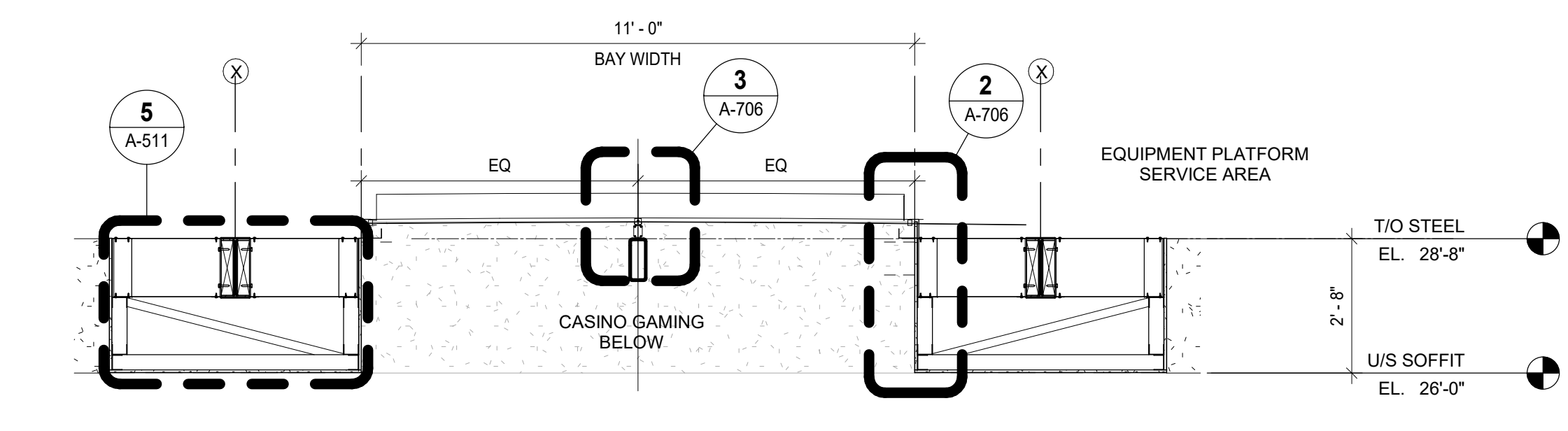
DETAIL - SECTION - RETRACTABLE CANOPY - WIDTH TYPE 1 AND TYPE 2
