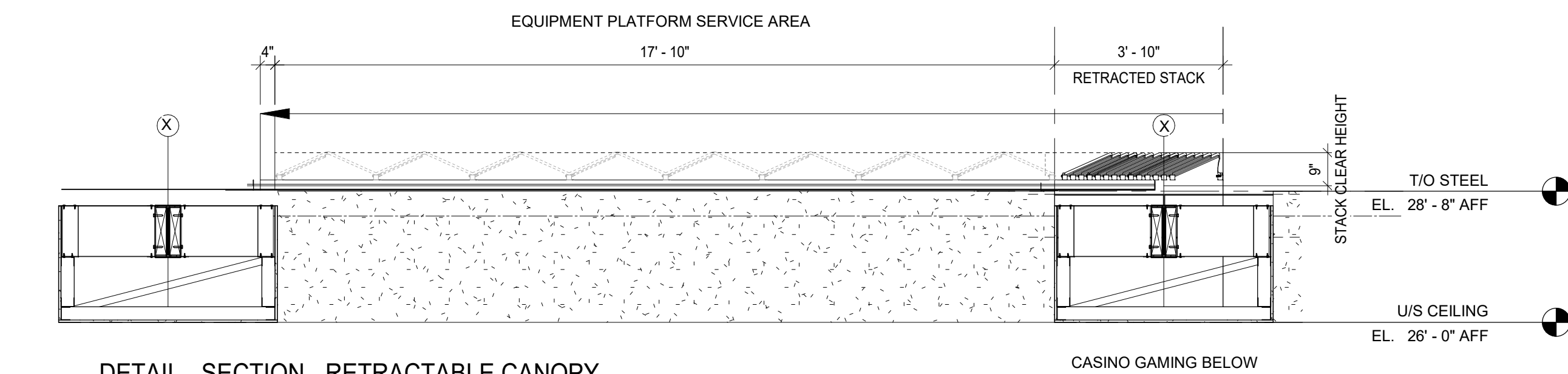
DETAIL - SECTION - RETRACTABLE CANOPY - LENGTH TYPE 1 AND TYPE 3
