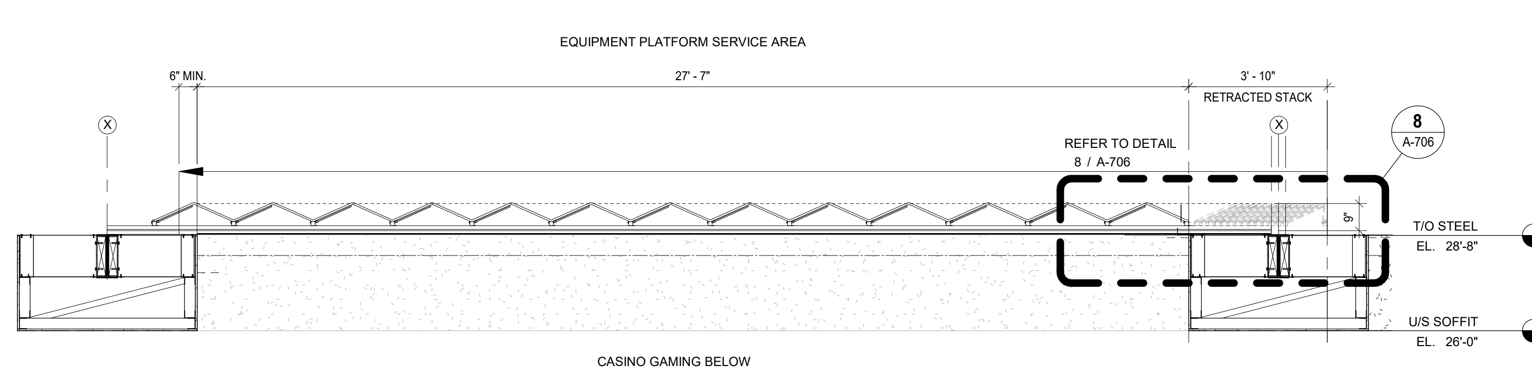
DETAIL - SECTION - RETRACTABLE CANOPY - LENGTH TYPE 2 AND TYPE 4
