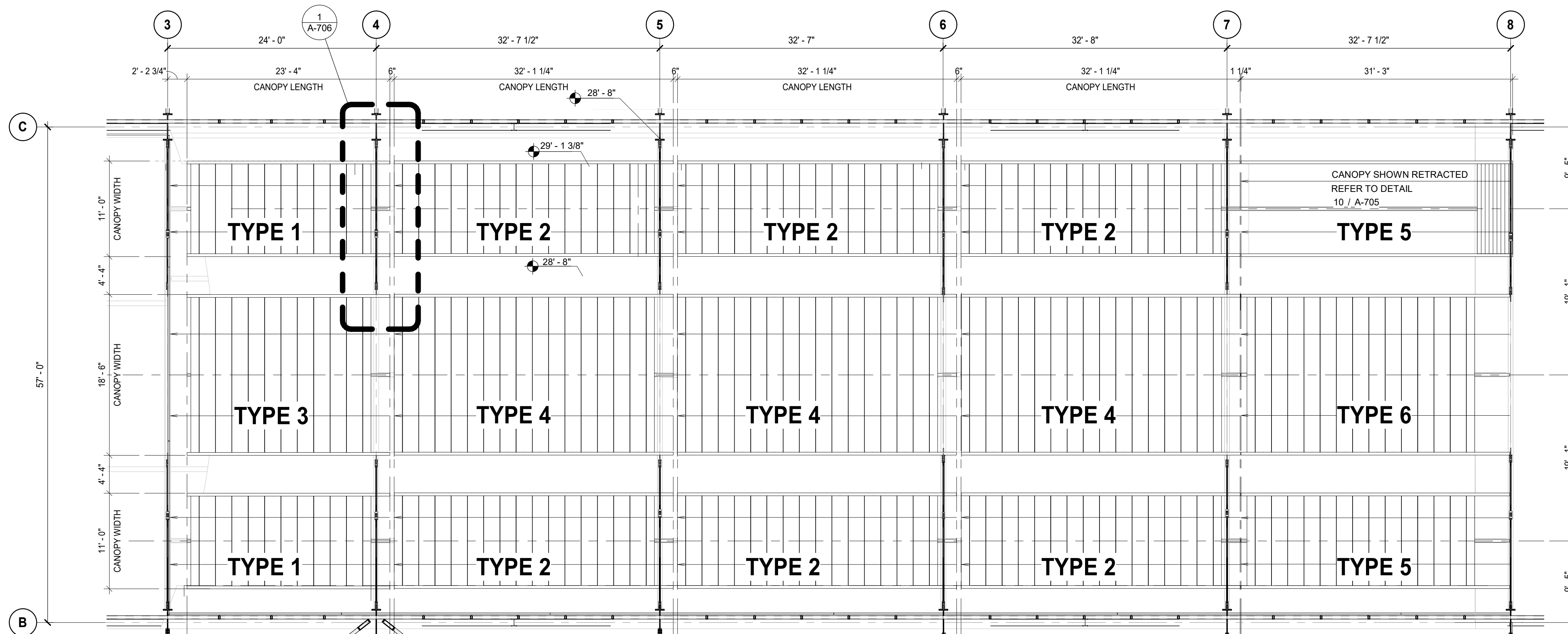
KEYPLAN - CANOPIES EXTENDED (DAY MODE)
