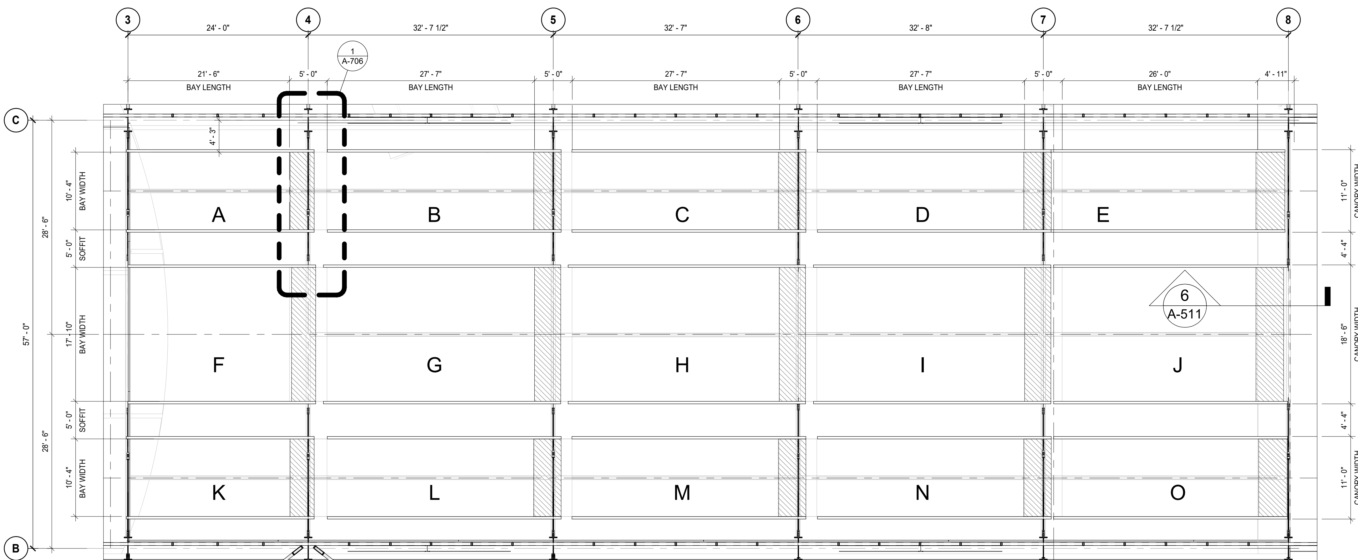
KEYPLAN - CANOPIES RETRACTED (NIGHT MODE)
