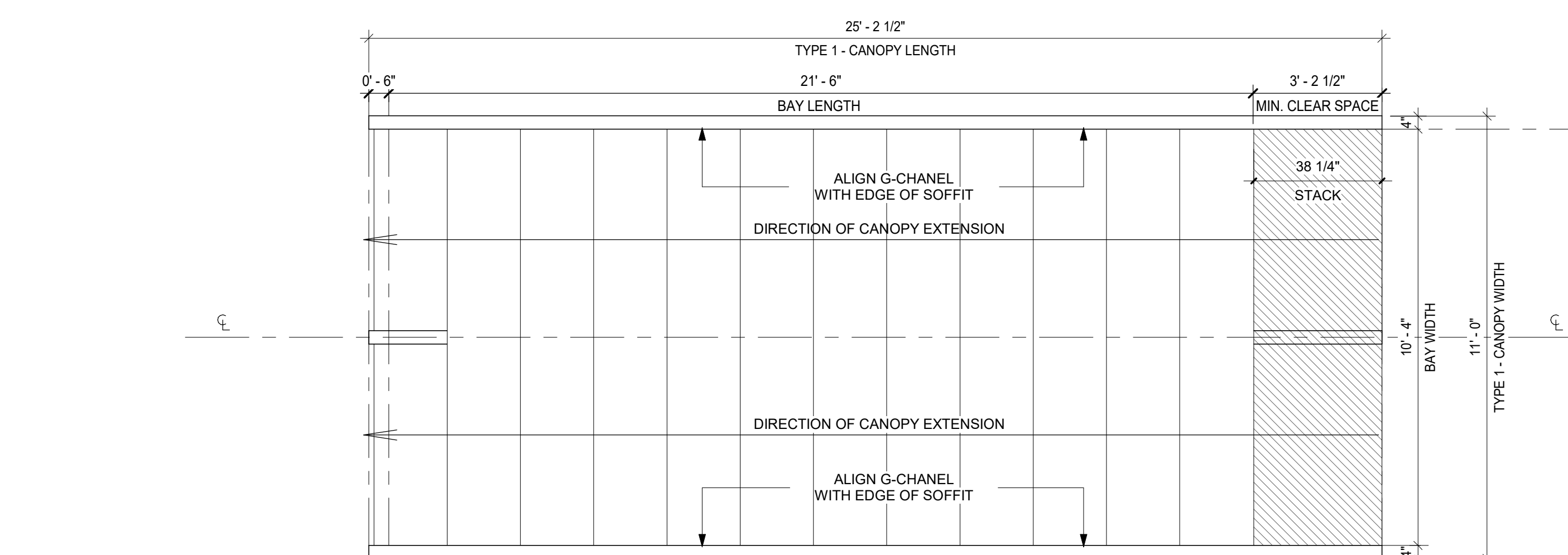
DETAIL - PLAN DIAGRAM - CANOPY TYPE 1
