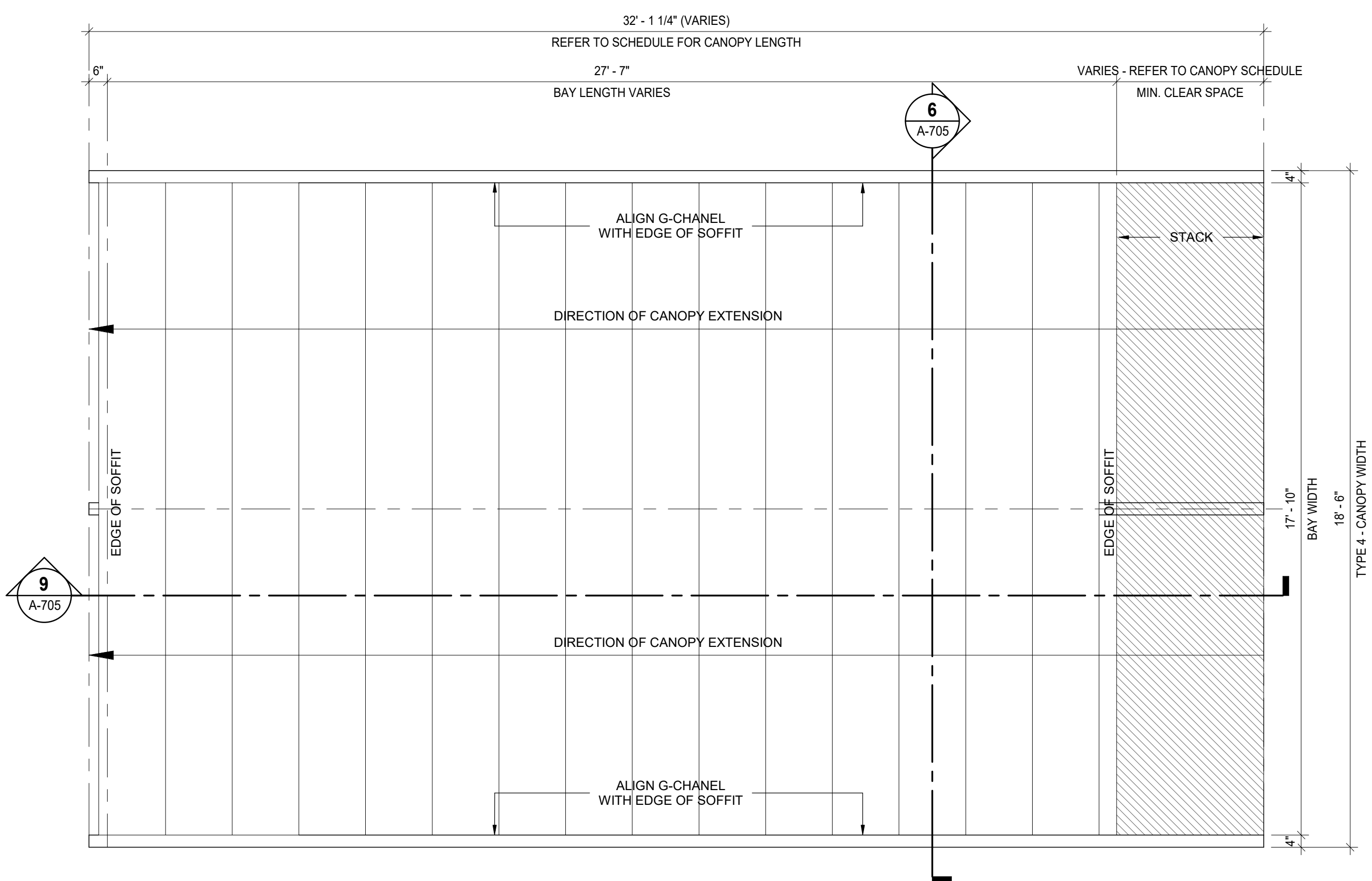
DETAIL - PLAN - SHADEFX CANOPY - TYPES 3, 4 & 6
