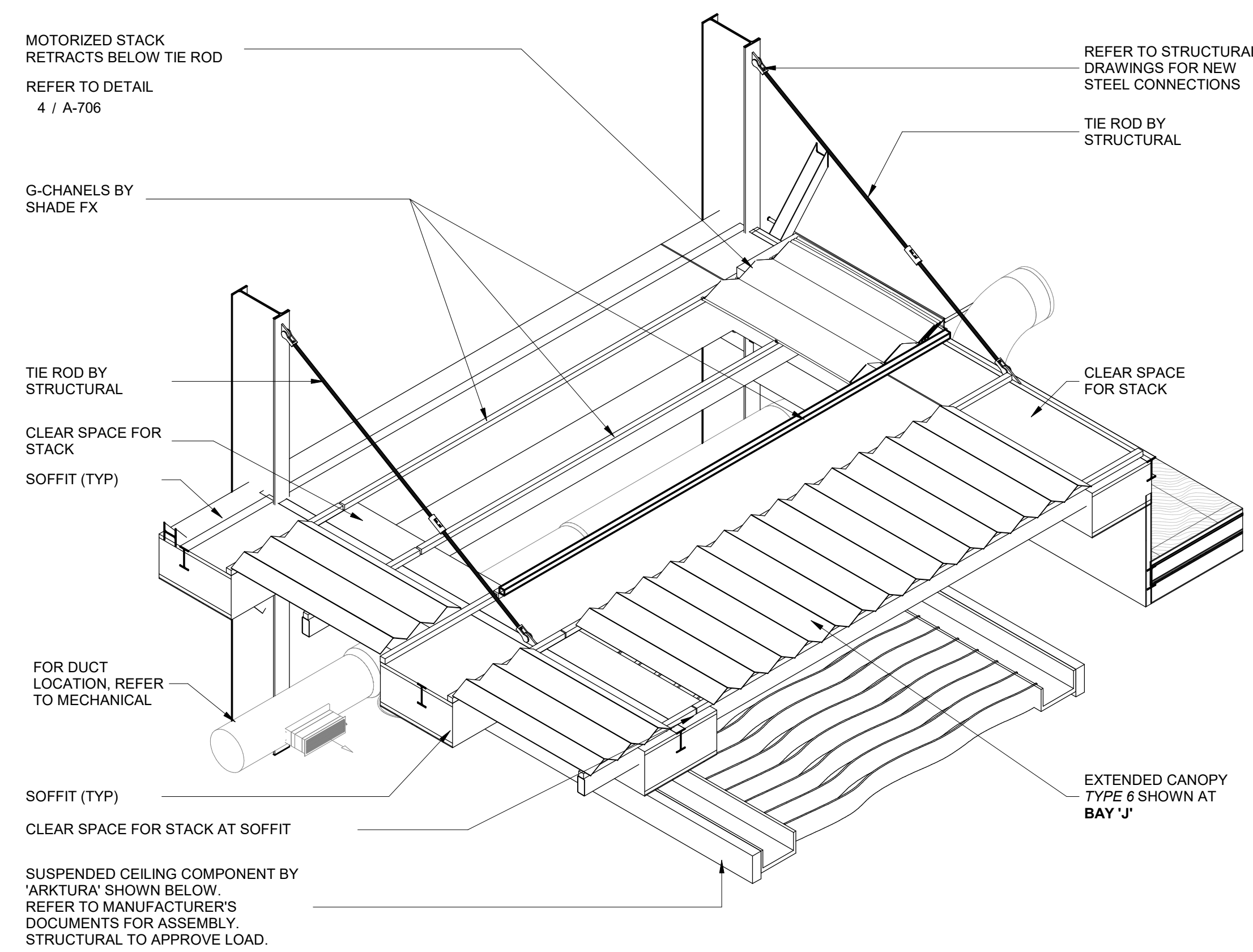
DETAIL ISOMETRIC - SHADEFX RETRACTABLE CANOPY
